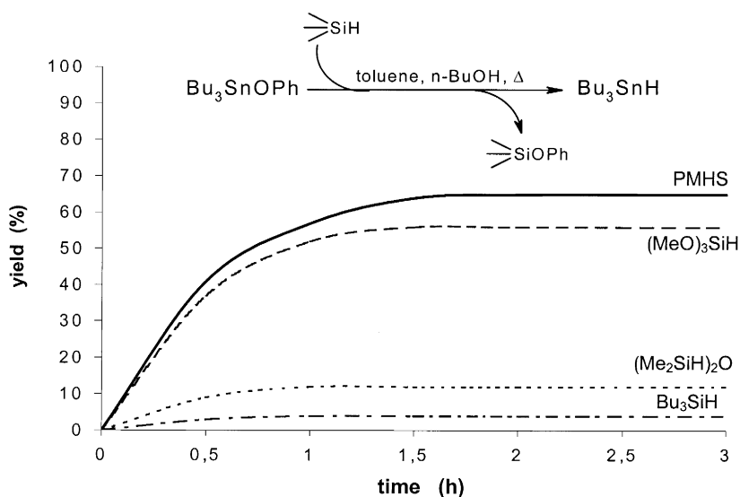
Fig. 1. Reduction of phenoxystributyltin by an hydrosil(ox)ane: \text{Bu}_3\text{SnH} formation monitored by gas chromatography. Reaction conditions: see the general procedure in Ref. 13
